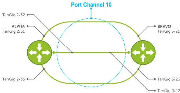
Figure 55. LACP Basic Configuration Example
